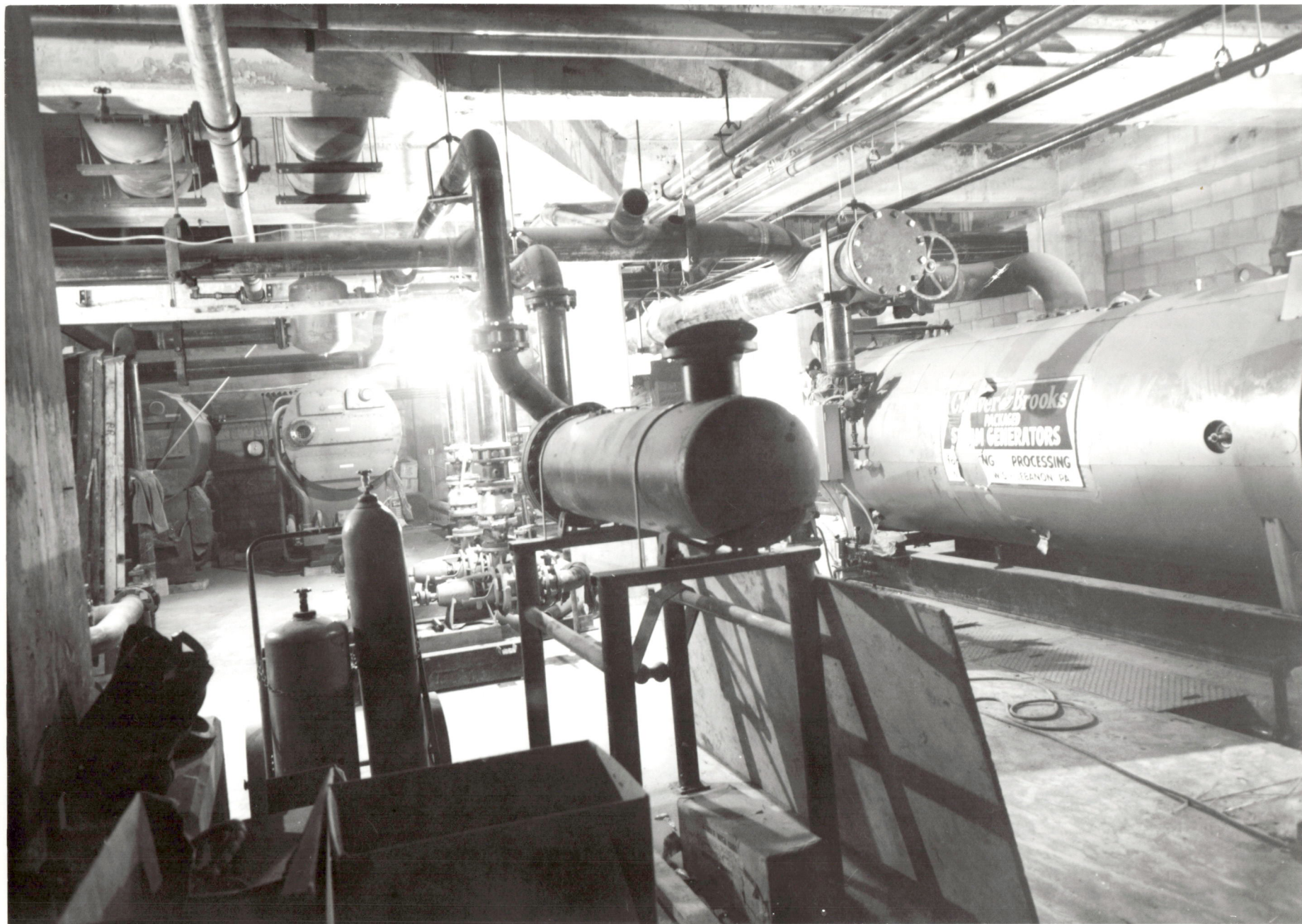
ACADEMIC CENTER UNIVERSITY OF BALTIMORE ROY KIRBY & SONS, INC., CONTRACTOR FISHER, NES, CAMPBELL & PARTNERS, ARCHITECTS BOILER JUNE 1, 1971
